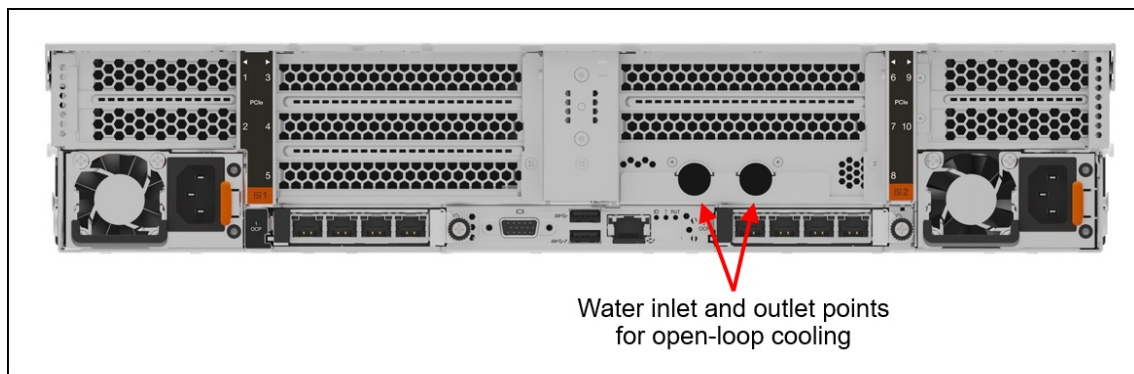
Figure 5. Rear of the SR650 V4 with open-loop water cooling
