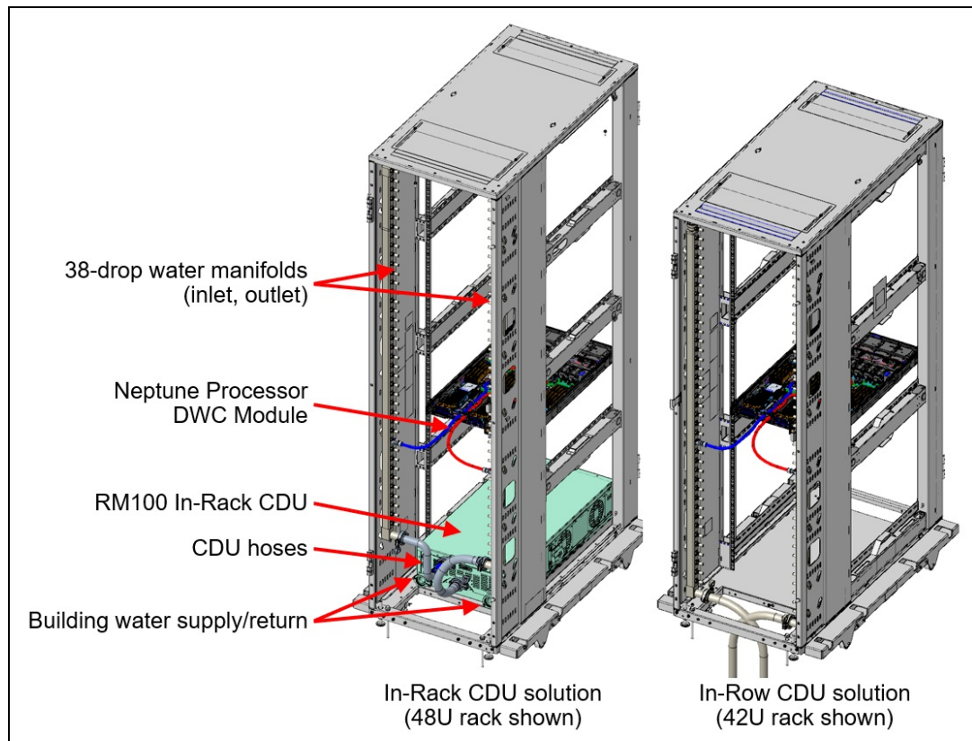
Figure 37. Water manifold connections
