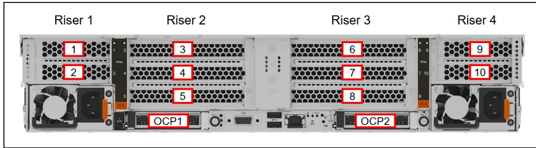
Figure 24. SR650 V4 rear slots
