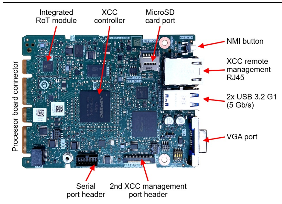
Figure 32. System I/O Board
