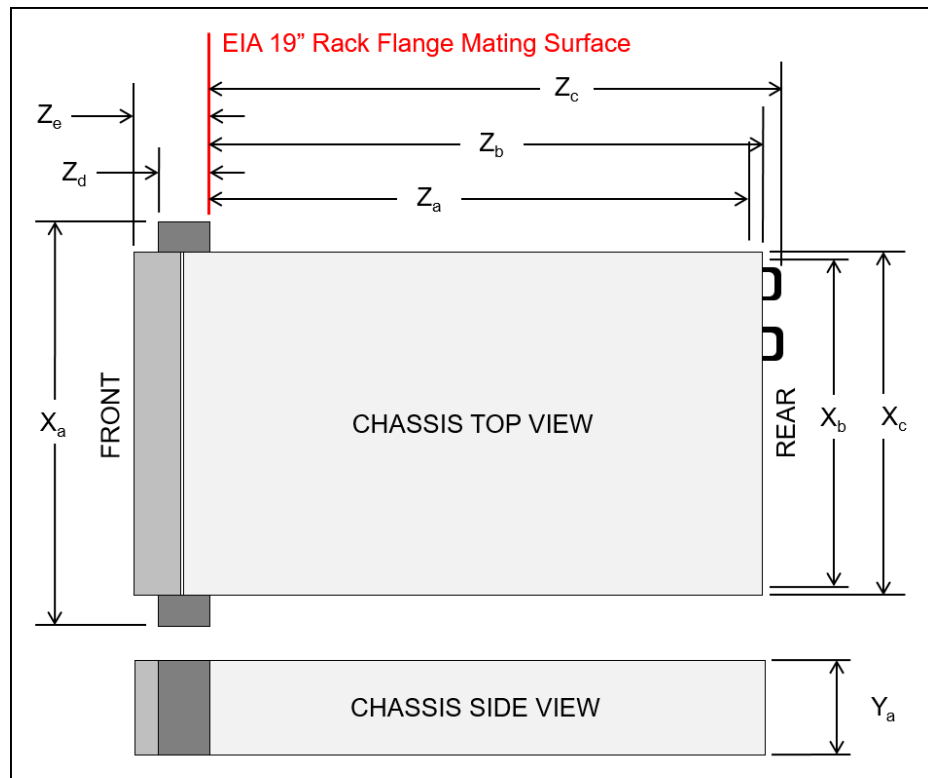
Figure 36. Server dimensions
